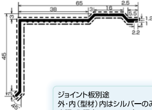
MT-42BS
