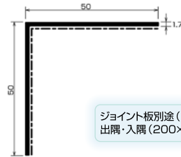
MT-50BC
