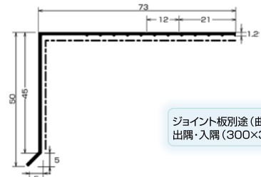
MT-50AS
