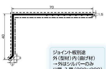
MT-40BS
