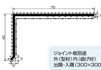
MT-40DS
