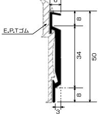
MC-50S
