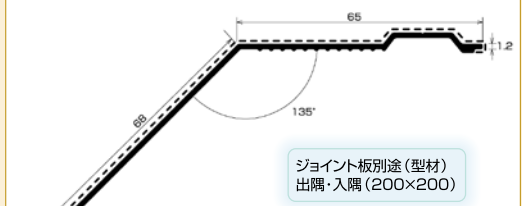
MT-50AB
