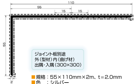
MT-55D
