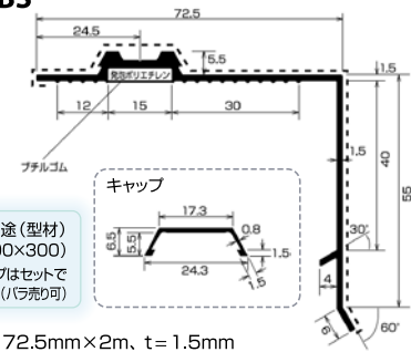
MT-50AS
